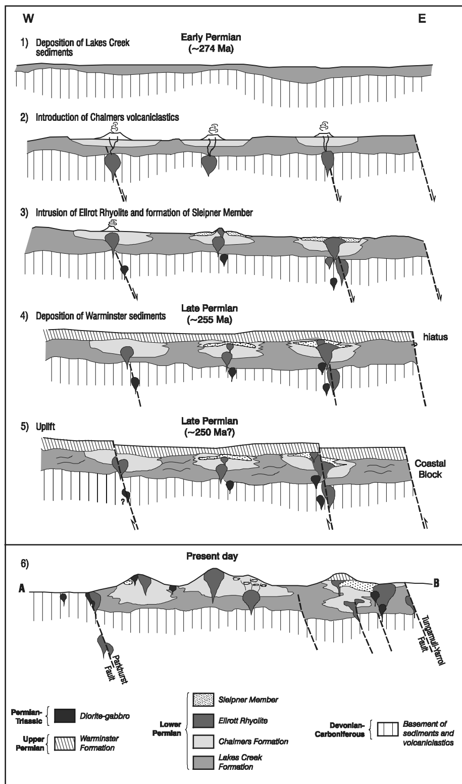
Figure 1: Schematic sections depicting the formation of units identified in the Rockhampton region. (Present day section A-B is defined on Map1)
